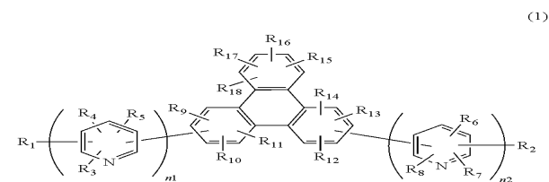
[Chemical Formula 1]
