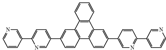
[Chemical Formula 12]
