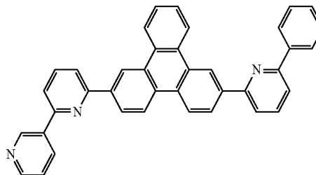
[Chemical Formula 15]
