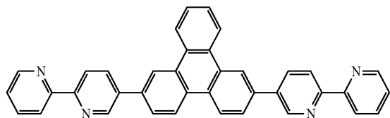
[Chemical Formula 8]
