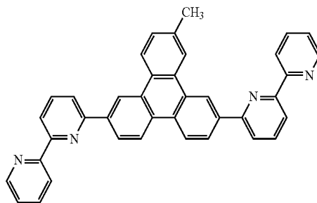
[Chemical Formula 13]
