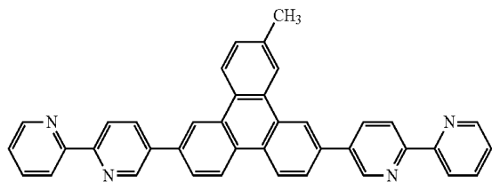
[Chemical Formula 10]
