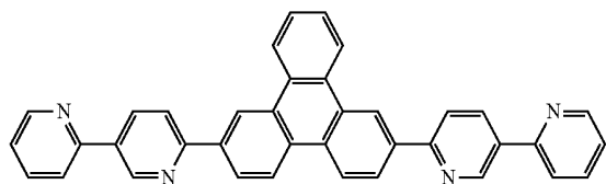
[Chemical Formula 14]
